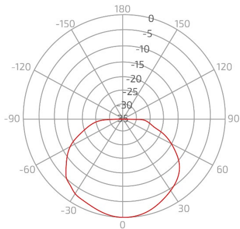
Elevation - SH-5800-10-90-DP
