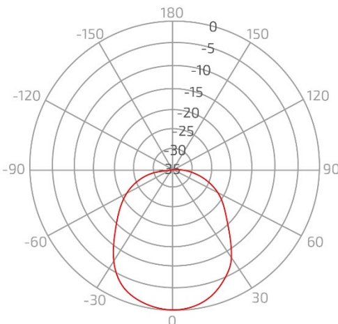
Elevation - SH-5800-13-60-DP
