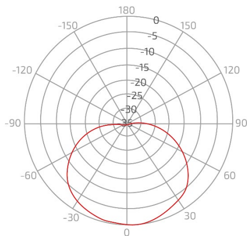
Elevation - SH-5800-10-90-DP
