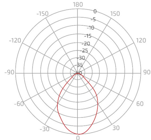
Elevation - SH-5800-18-30-DP
