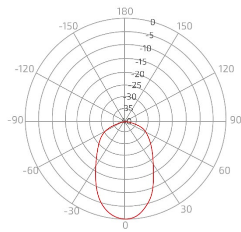
Elevation - SH-5800-18-30-DP
