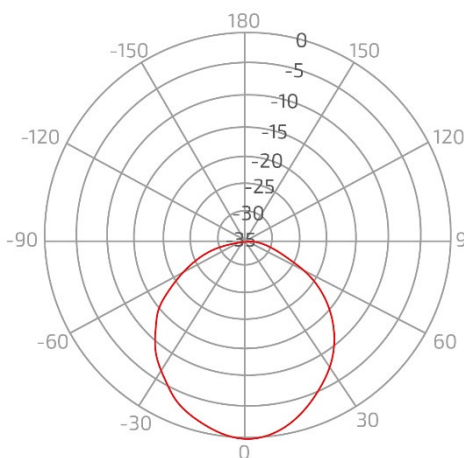
Elevation - SH-5800-13-60-DP
